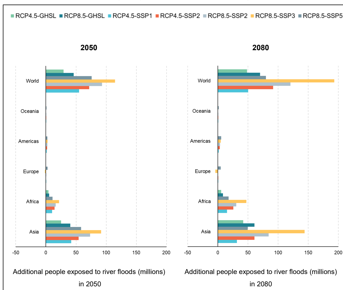
Figure 14. The projected people exposed to river floods in 2050 and 2080 stratified by emissions and socioeconomic scenario combination. The bars indicate the projected additional people for each scenario relative to the baseline (ensemble mean of 1971-1999 historical flood hazard and GHSL 2015 population layer). SSPs include SSP1 (Sustainability - low challenges to mitigation and adaptation), SSP2 (Middle of the road - medium challenges to mitigation and adaptation), SSP3 (Regional rivalry - high challenges to mitigation and adaptation, SSP5 (Fossil fuel development - high challenges to mitigation with low challenges to adaptation). RCP=representative concentration pathways, SSP=shared socioeconomic pathways, GHSL=Global Human Settlement layer 2015.
