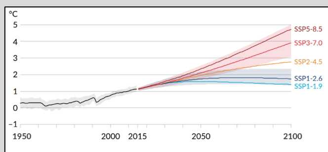
Figure B1: Global surface temperature change relative to 1850–1900
