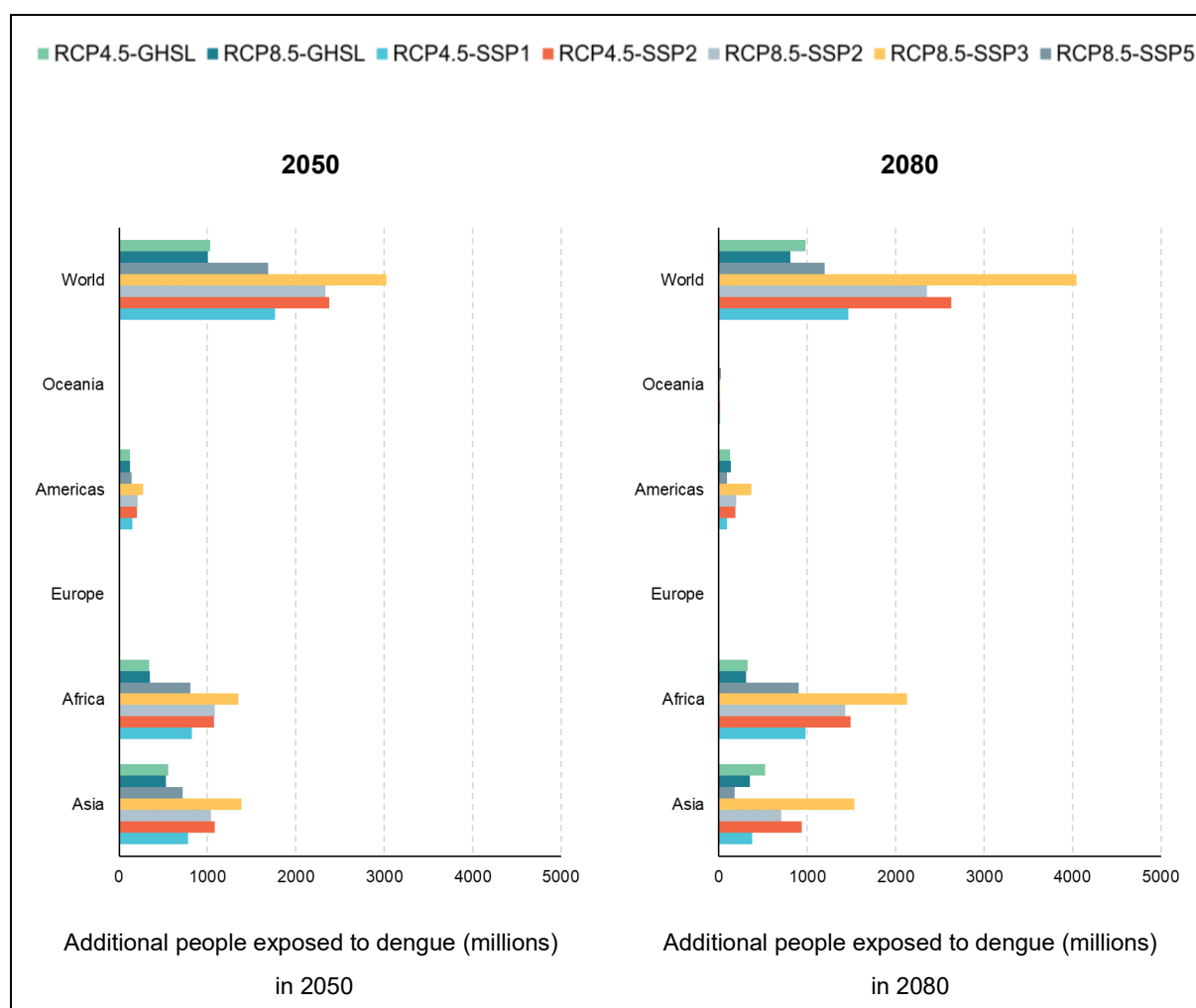
Figure 18. The projected people exposed to dengue in 2050 and 2080 stratified by emissions and socioeconomic scenario combination. The bars indicate the projected additional people for each scenario relative to the baseline (ensemble mean of 1970-1999 historical period and GHSL 2015 population layer). SSPs include SSP1 (Sustainability - low challenges to mitigation and adaptation), SSP2 (Middle of the road - medium challenges to mitigation and adaptation), SSP3 (Regional rivalry - high challenges to mitigation and adaptation), SSP5 (Fossil fuel development - high challenges to mitigation with low challenges to adaptation). RCP=representative concentration pathways, SSP=shared socioeconomic pathways, GHSL=Global Human Settlement layer 2015.
