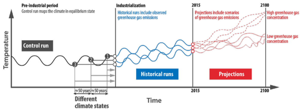
Figure 3. Schematic representation of a climate projection. Modified from DWD (2021)
